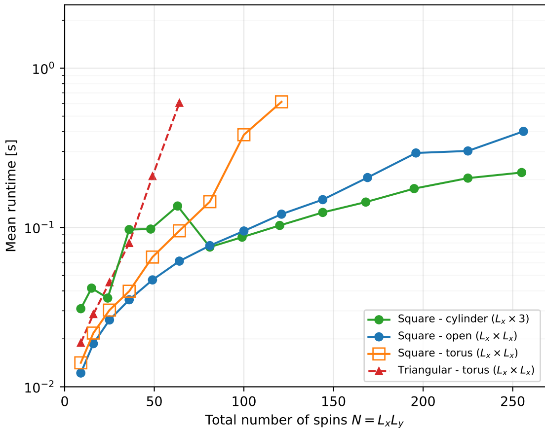
Runtime for Z using TensorOrder
